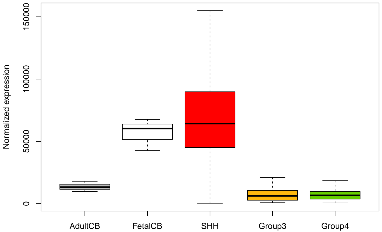
SEMA6A ENSG00000092421 expression (no outliers)
