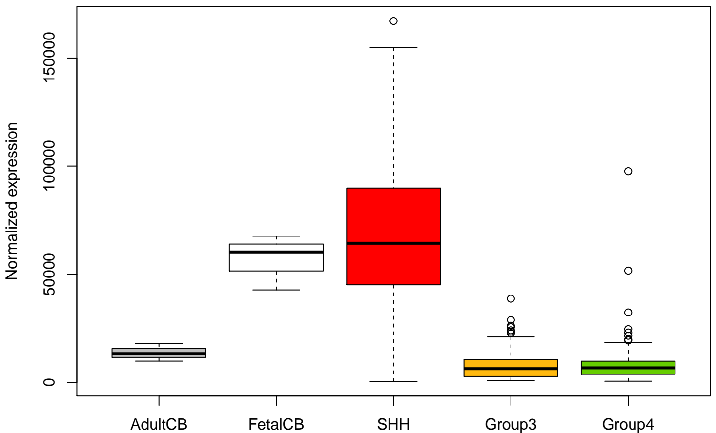
SEMA6A ENSG00000092421 expression (including outliers)
