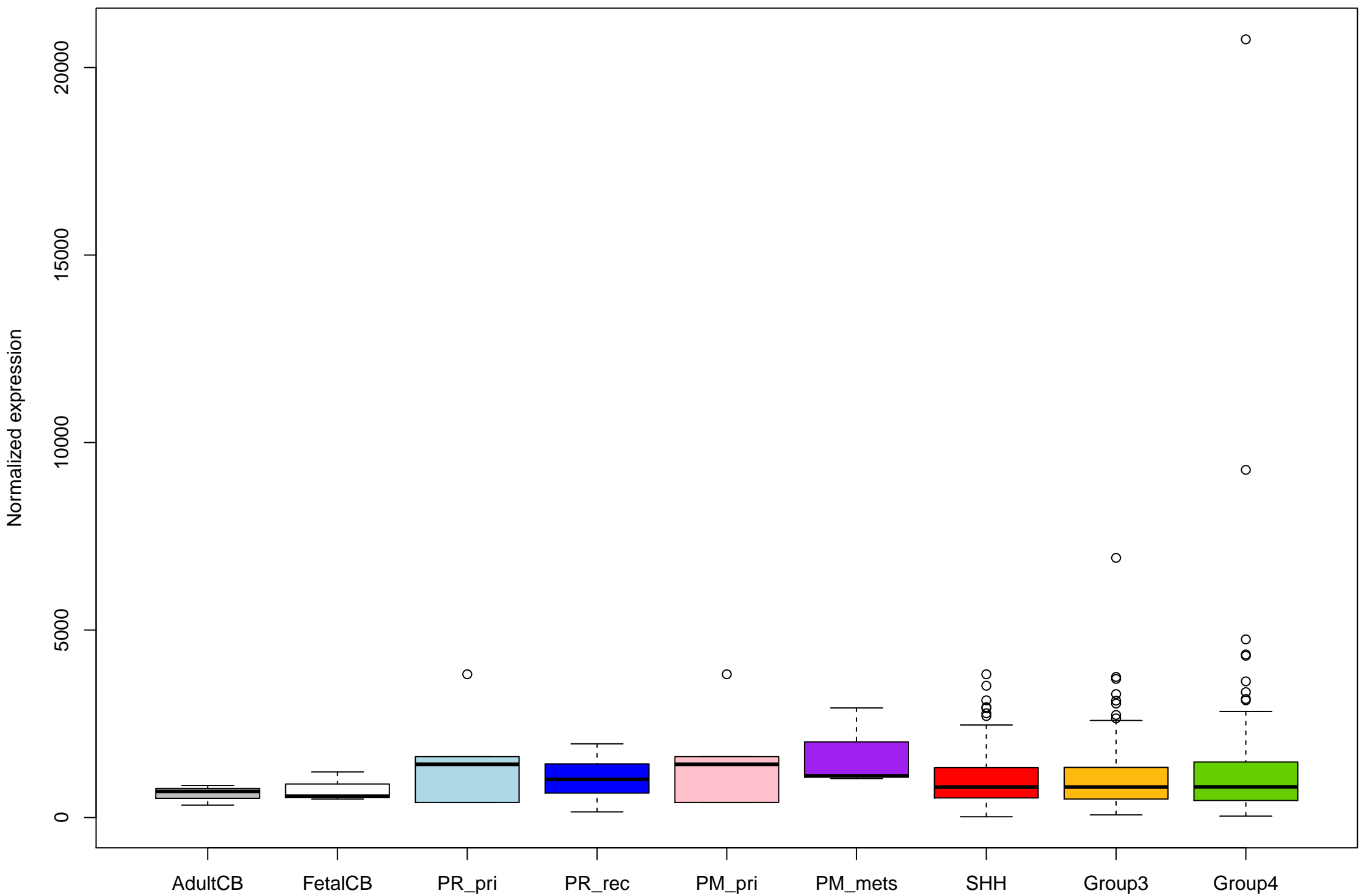
ENSG00000206190_ATP10A_ – expression (with outliers)
