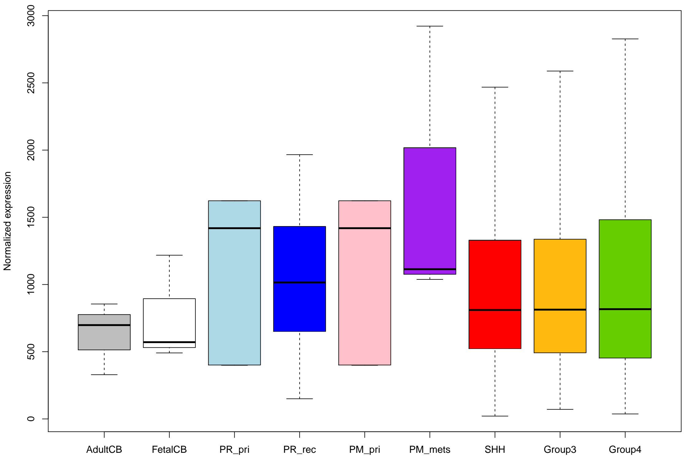
ENSG00000206190_ATP10A_ – expression (no outliers)
