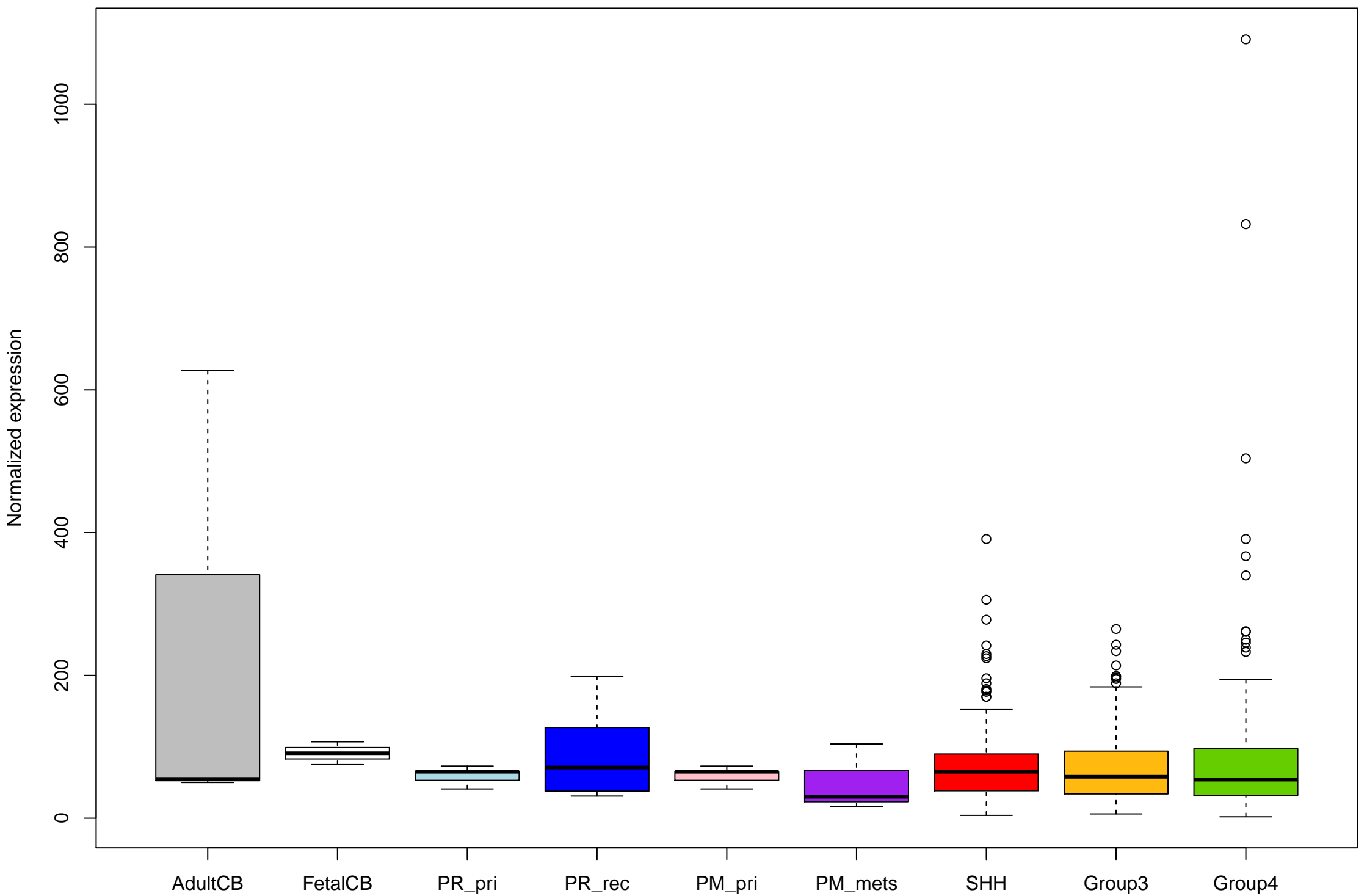
ENSG00000196196_HRCT1_+ expression (with outliers)
