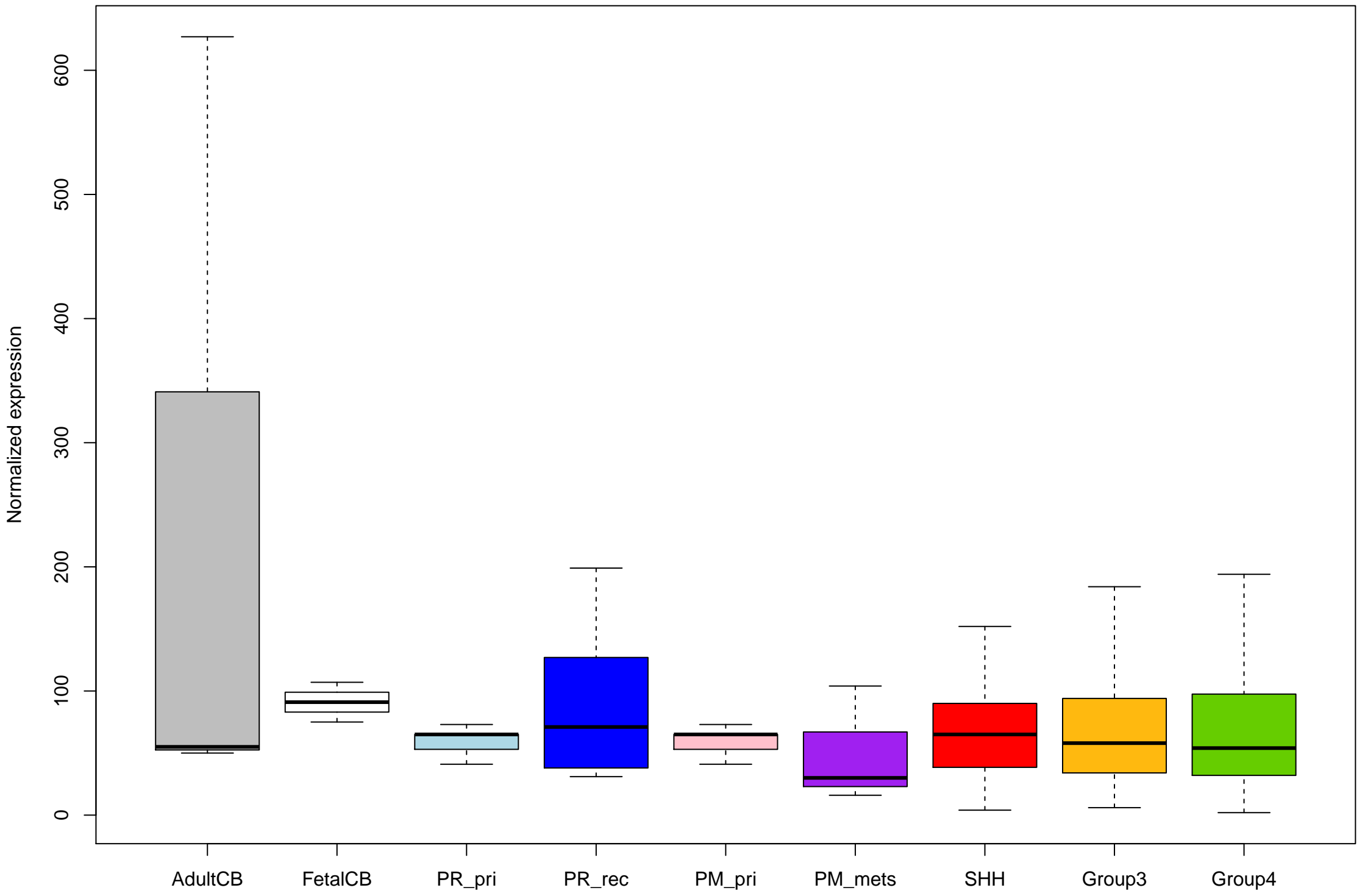
ENSG00000196196_HRCT1_+ expression (no outliers)
