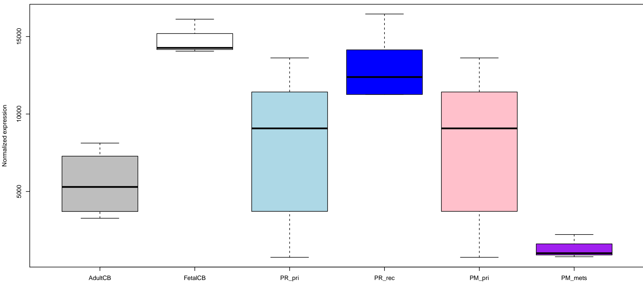
NOTCH2_expression (no outliers)
