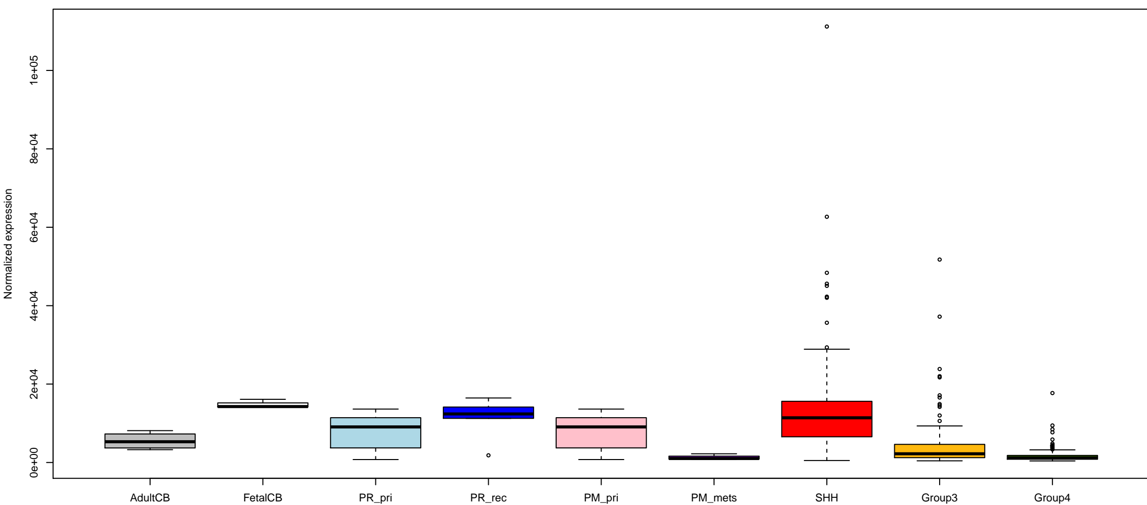
NOTCH2_expression (with outliers)
