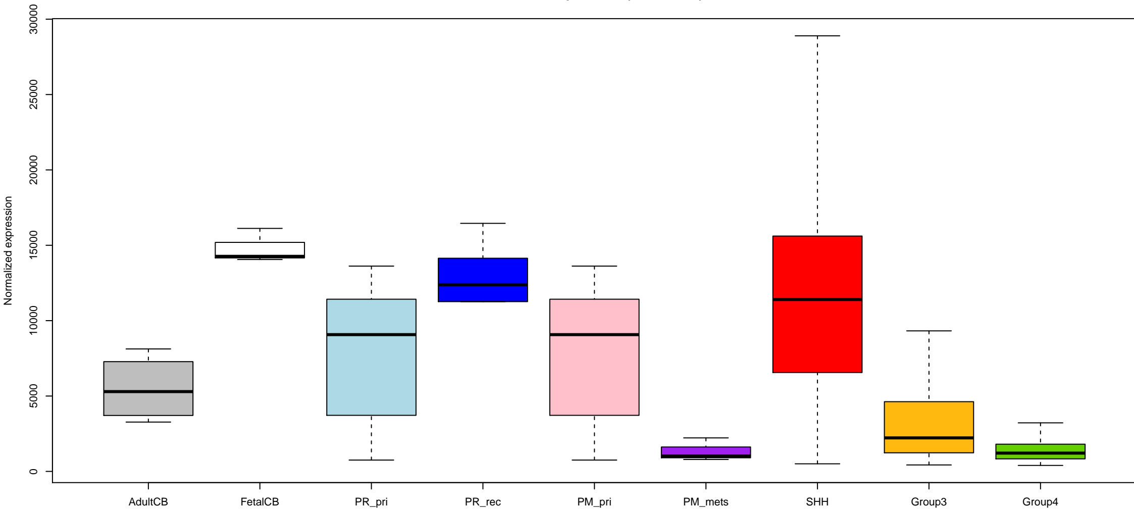
NOTCH2_expression (no outliers)
