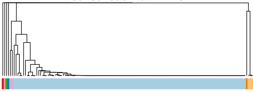
consensus matrix k=8
