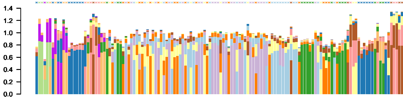
item-consensus k=11
