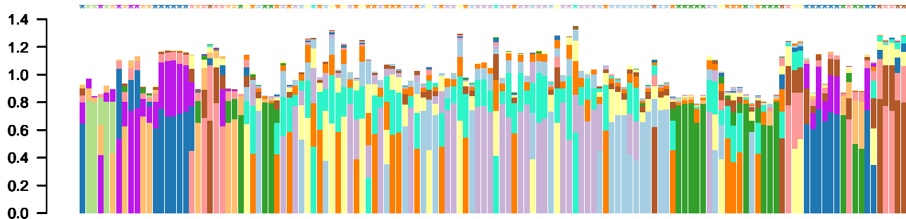
item-consensus k=12
