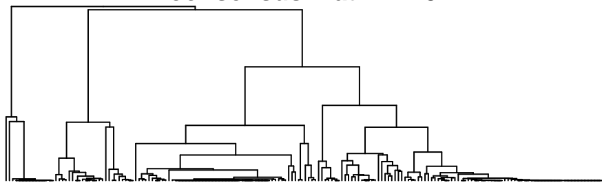
consensus matrix k=3
