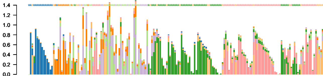
item-consensus k=7
