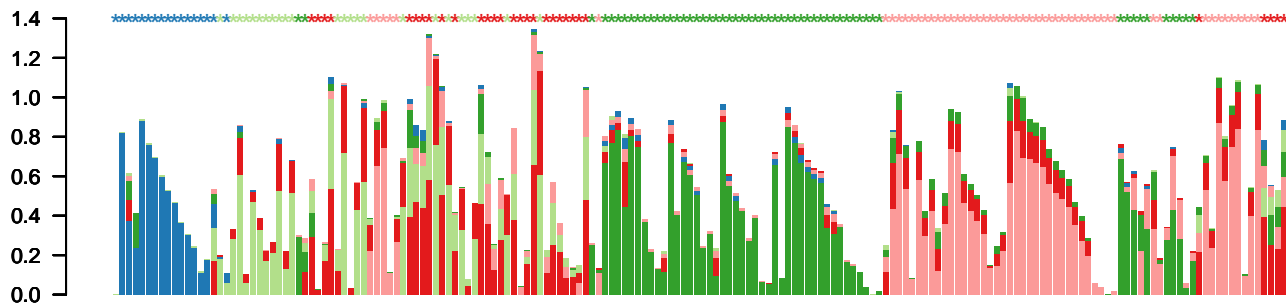
item-consensus k=5
