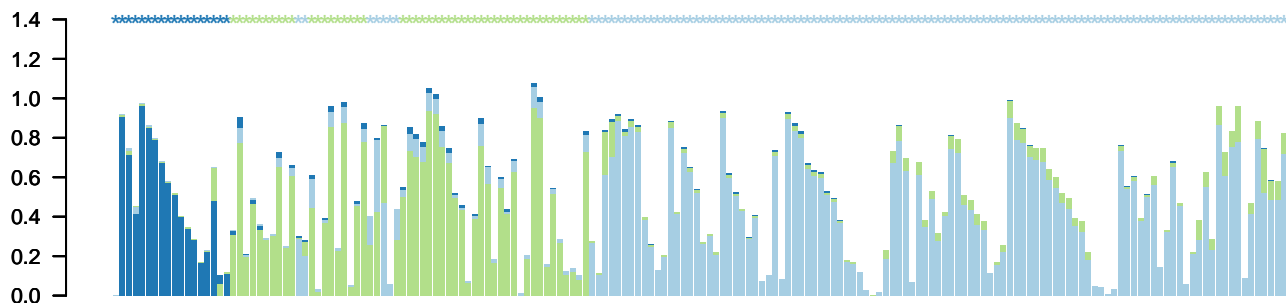
item-consensus k=3
