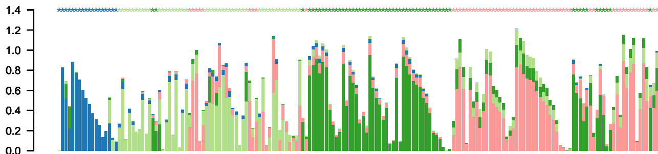
item-consensus k=4
