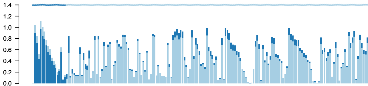
item-consensus k=2
