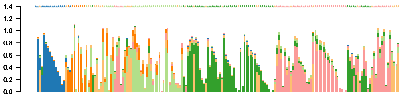
item-consensus k=6
