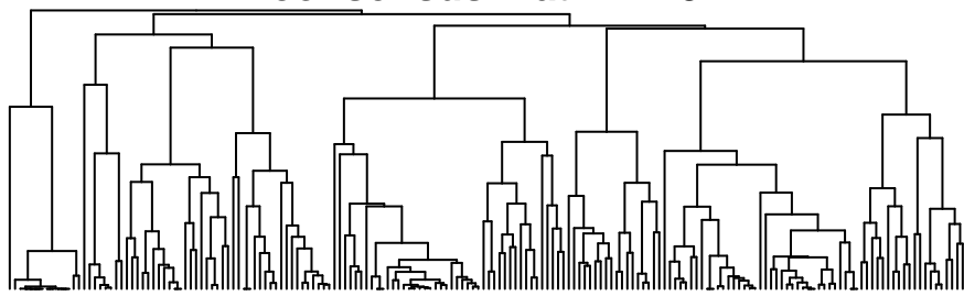
consensus matrix k=9
