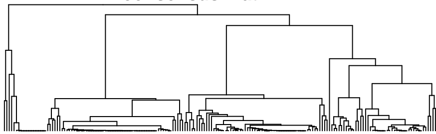
consensus matrix k=4
